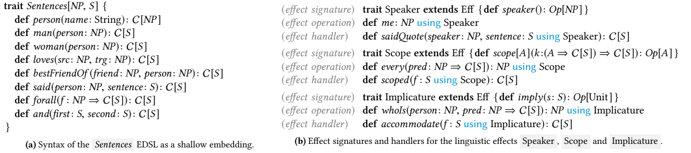
Figure 1. Syntax of the Sentences EDSL and the interface for linguistic effects.
